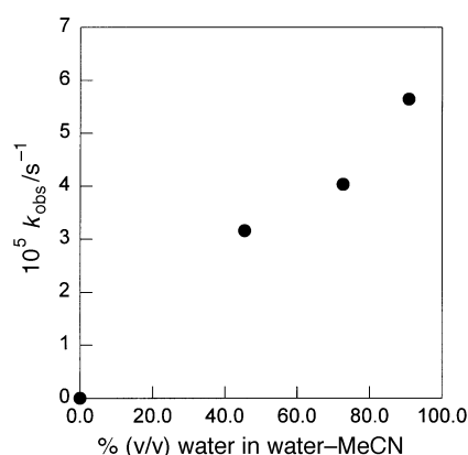
Fig. 5 Relationship between k_{\text{obs}} and the volume fraction of water in the water-MeCN mixture at 50 °C and I = 0.1 mol dm -3 ( \text{LiClO}_4 )
