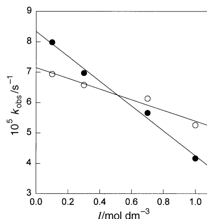
Fig. 6 Relationship between k_{\text{obs}} and ionic strength ( I ) in an aqueous solution containing 9.1% (v/v) MeCN at 50 °C and pH 7.0 ([hepes] = 0.05 mol dm -3 ): (●) \text{LiClO}_4 , (○) \text{LiO}_3\text{SCF}_3
