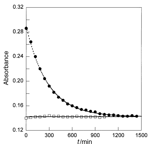
Fig. 4 Absorbance changes of (R,S,R,S) - (●) and (R,R,S,S) - [\text{NiL}][\text{ClO}_4]_2 (□) at 505 nm in an aqueous solution containing 9.1% (v/v) MeCN: [complex] = 2.86 mmol dm -3 , 50 °C, I = 0.1 mol dm -3 ( \text{KCl} ). Dashed line is the best-fit curve for the pseudo-first-order reaction with k_{\text{obs}} = (5.90 \pm 0.09) \times 10^{-5} \text{ s}^{-1}
