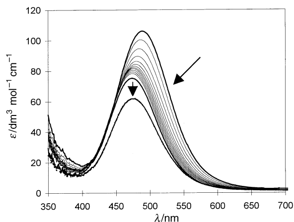
Fig. 3 Spectral changes of (R,S,R,S) - [\text{NiL}][\text{ClO}_4]_2 at 50 °C in an aqueous solution containing 9.1% (v/v) MeCN, at pH 7.0 ([hepes] = 0.05 mol dm -3 ) and I = 0.1 mol dm -3 ( \text{LiClO}_4 ). Spectra were recorded every 2 h and the final spectrum 30 h after the start. The vertical arrow represents the final spectrum measured at 25 °C
