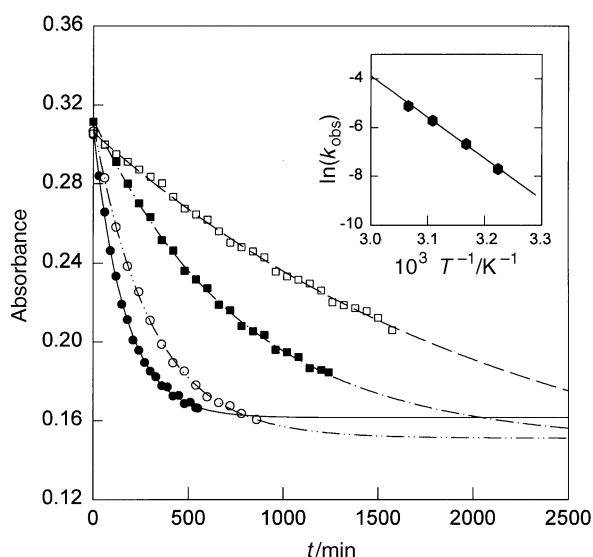
Fig. 7 Temperature dependence of the absorbance change for (R,S,R,S)\text{-}[\text{NiL}][\text{ClO}_4]_2 in an aqueous solution containing 9.1% (v/v) MeCN at 505 nm, pH 7.0 ( [\text{hepes}] = 0.05 \text{ mol dm}^{-3} , I = 0.1 \text{ mol dm}^{-3} ( \text{LiClO}_4 )): 326 (●), 321 (○), 315 (■) and 310 K (□). Inset: Arrhenius plot
